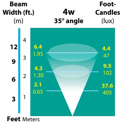
35° MR16 LED
