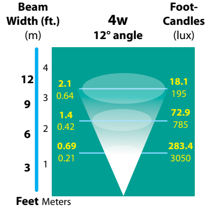
12° MR16 LED
